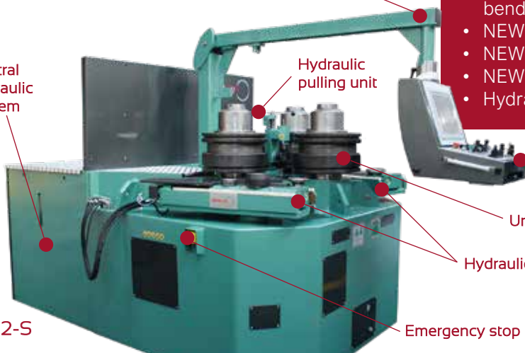
Swing-arm
