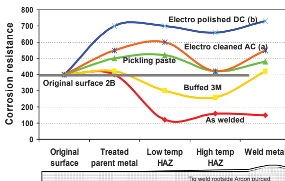
Figure 4. Effect of cleaning methods on a stainless steel weldment
